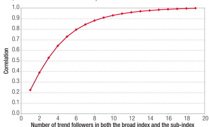
Correlation between returns on a sub-index of correlated returns and a broader index
